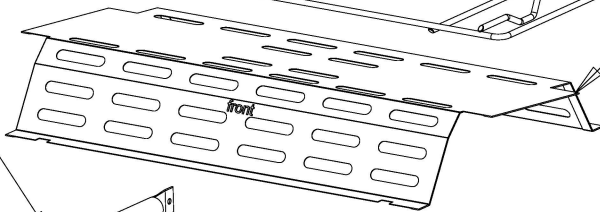
BURNER (1) PZOVEN-5
